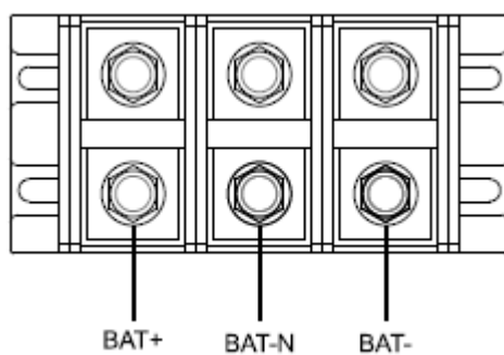
G33-HV 60KL/80KL and G33-LV 30KL/40KL 端子排示意图
