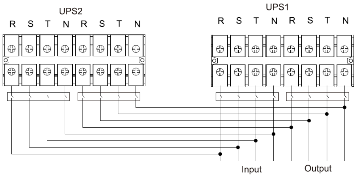
G33-HV 60KL/80KL and G33-LV 30KL/40KL 并机系统接线图
